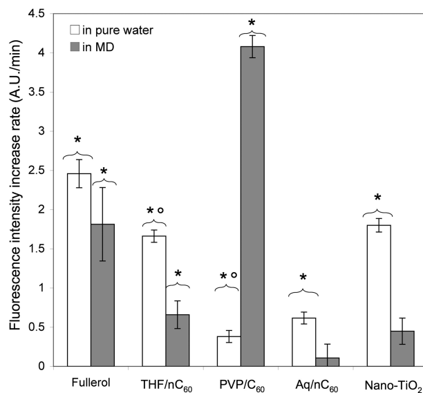
FIGURE 3. Differences in singlet oxygen production by different nanoparticle suspensions (25 \mu\text{M} each) exposed to UV in ultrapure water or in MD. Generation of \text{O}_2^{\cdot-} was assessed per SOSG fluorescence. Bars indicate the standard deviation of the mean ( n = 3 ). * denotes a significant difference from the control at the 95% confidence level. THF/nC 60 and PVP/C 60 induced a drop in pH (pH \sim 4 ) that deactivated the SOSG dye.
