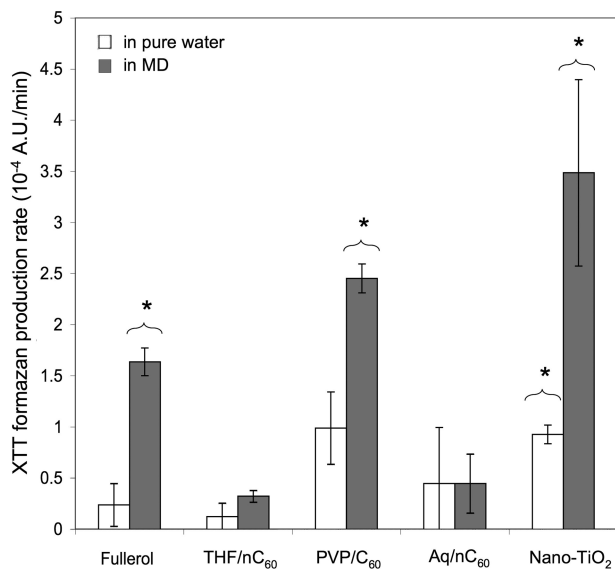
FIGURE 2. Superoxide production by different nanoparticle suspensions (5 \mu\text{M} each) exposed to UV in ultrapure water or in MD. Generation of \text{O}_2^{\cdot-} was assessed per XTT-formazan production, measured as increase in absorbance at 470 nm. Bars indicate the standard deviation from the mean ( n = 3 ). * denotes a significant difference from the control at the 95% confidence level.
